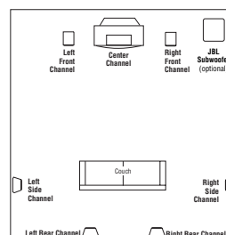
Figure 5. This overhead view shows a typical home theater plan when using two rear channel speakers.
